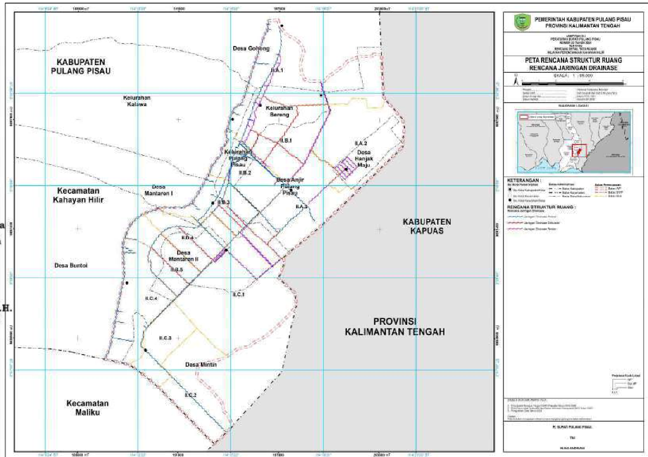
RENCANA JARINGAN DRAINASE WP KAHAYAN HILIR
